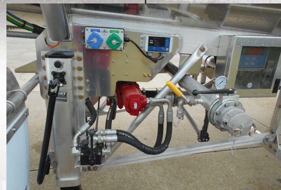
Control Box, Rack Controls, and Invert Mounted Roper Pump (Optional)
